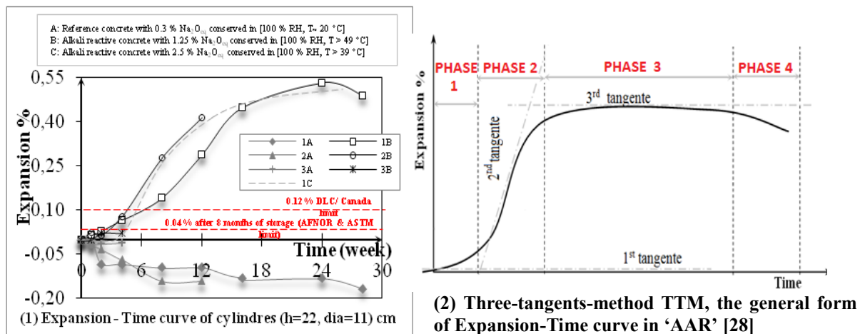
Figure.4: Expansion test with cylindrical samples (h 22, Ø 11) cm with (3B, 2B and 1B)
